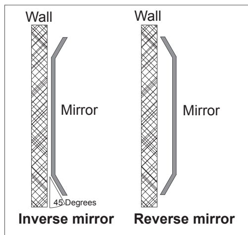
Cross Section of Angled Profile Mirror
